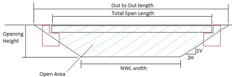
Figure 28 Typical Bridge Parameters
